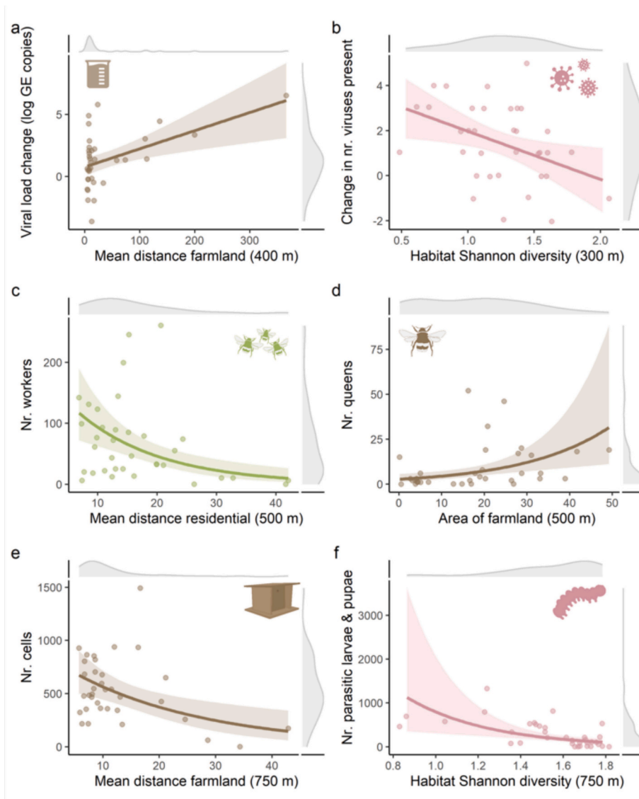
Fig. 3. Linear relationships between the landscape structure and changes in the bumble bee virome (a, b), and colony development parameters at the end of field placement(c-f). a) Change of total viral load (GE copies on log scale) and mean nearest-neighbor distance among farmland patches within 400 m radius, b) change in number of different viruses present and habitat Shannon diversity within 300 m radius around the bumble bee colonies, c) number of workers per colony and the mean nearest-neighbor distance of residential areas within 500 m, d) number of queens per colony and the relative area covered by farmland within 500 m, e) number of all cells per colony and mean nearest-neighbor distance among farmland patches within 750 m, and f) number of parasitic larvae and pupae per colony and habitat Shannon diversity within 750 m. Estimates are derived from the respective best model per response variable where other terms present in the model were set at their mean. Solid lines depict the estimated mean, shaded area the confidence interval and the points and density distributions at the right and top of the plot show the distribution of the raw data.
